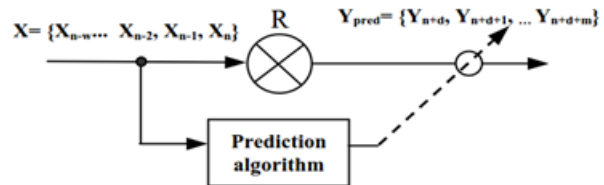
Fig. 3. Realization principle of bandwidth adaptive control.
