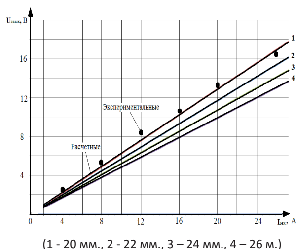
Fig.1 Steady-state features of output voltage under different FMW under importances of the air clearance ( points - an experiment, line – a design values)
