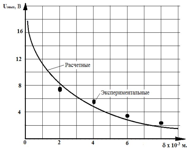
Fig.2. Dependency of the U_{\text{out}} with different importances
